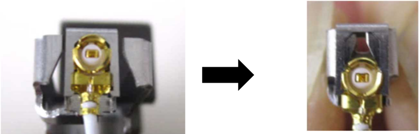
Clipping lock parts with unmating jig
