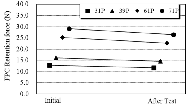
Graph.4 A change of FPC Retention force B group : FPC Retention force
