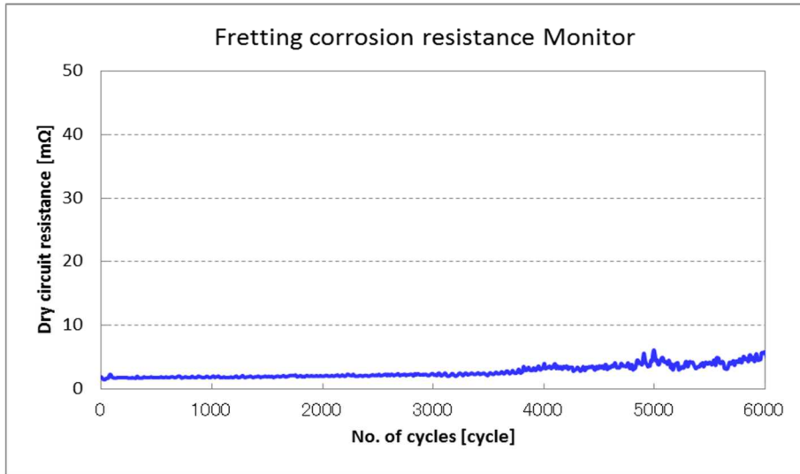
Grpf1. Fretting corrosion Resistance Monitor
