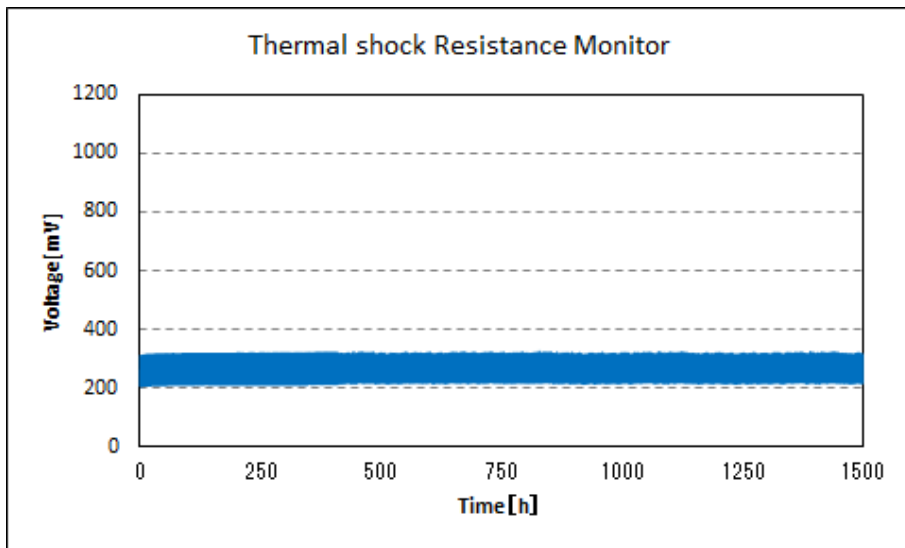
Graph2. Thermal shock Resistance Monitor
