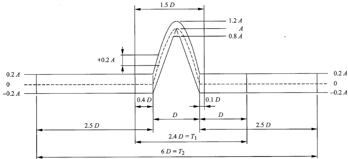
Fig.7 Sinusoidal half-wave
