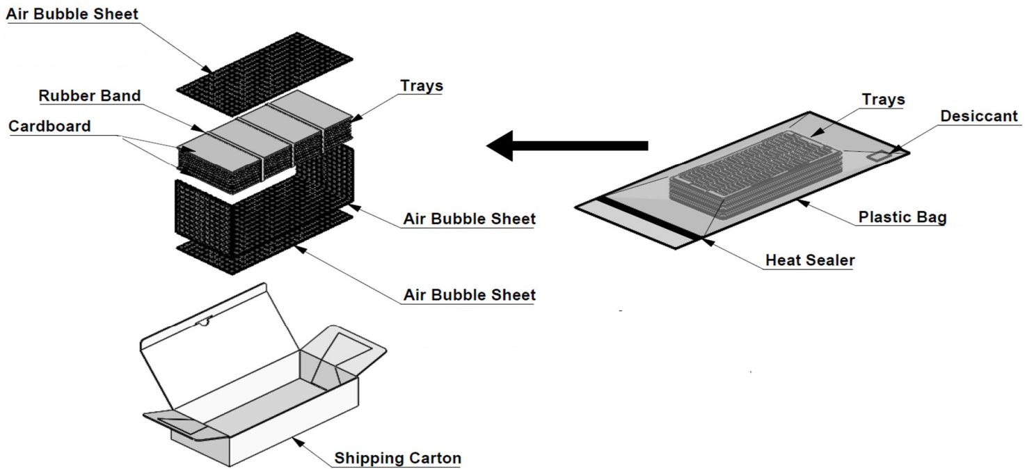
Fig. 2 Packing of Shipping Carton
