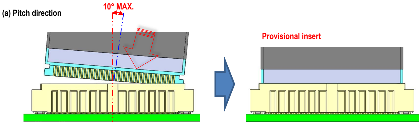
Fig.2-2 FFC/FPC insertion method 2
