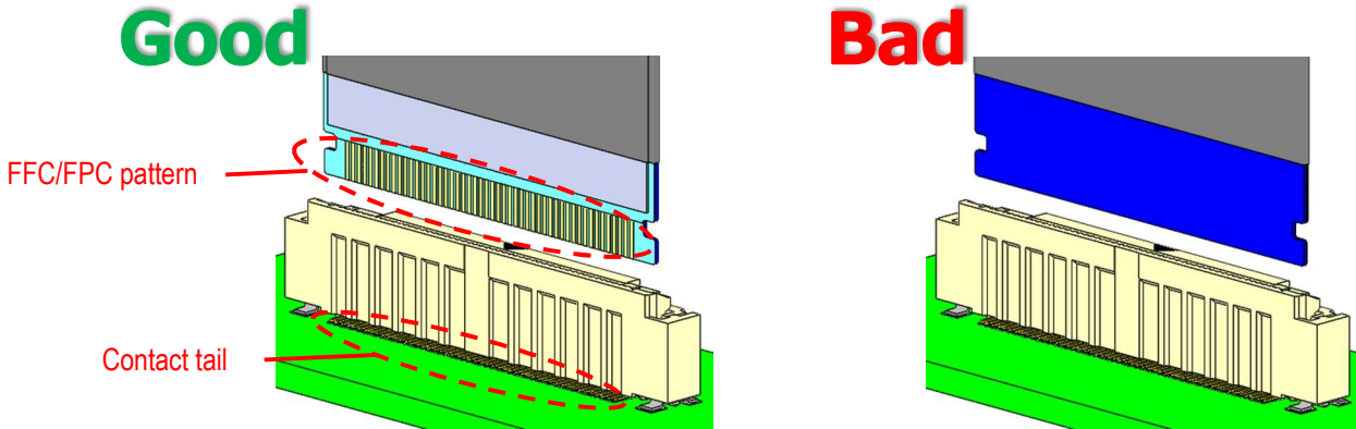
Fig.2-1 FFC/FPC insertion method 1
