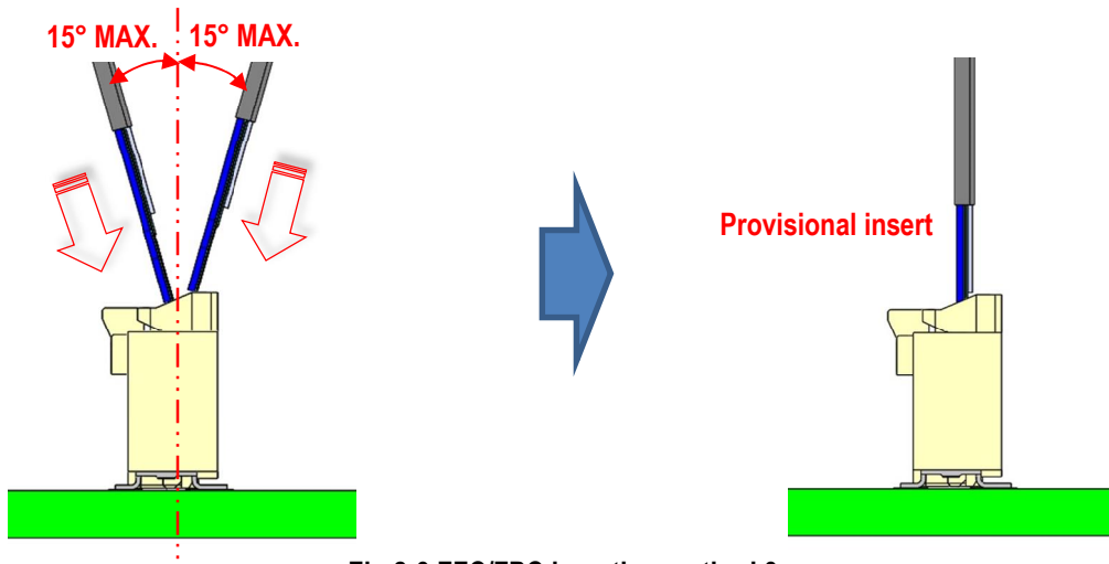
Fig.2-3 FFC/FPC insertion method 3
