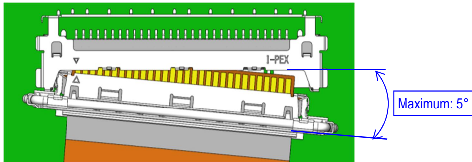
Fig. 5 Maximum Horizontal Insertion Angle
