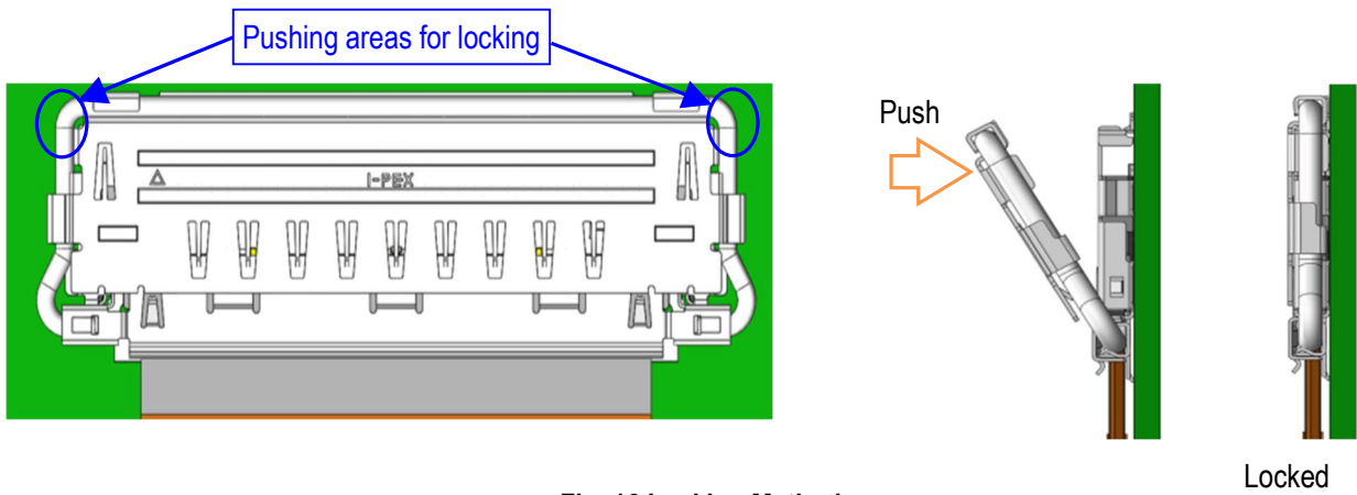
Fig. 16 Locking Method
