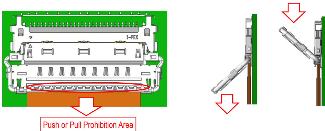
Fig. 23 Incorrect Removal Method
