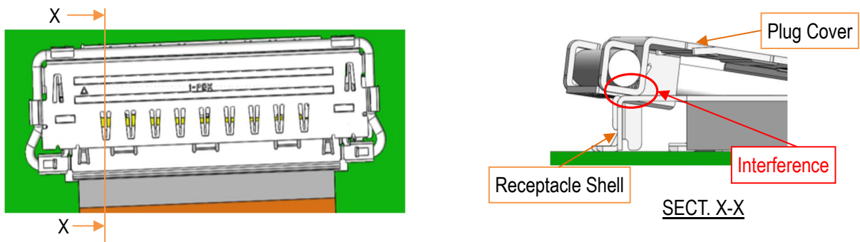
Fig. 9 Plug and Receptacle Interference
