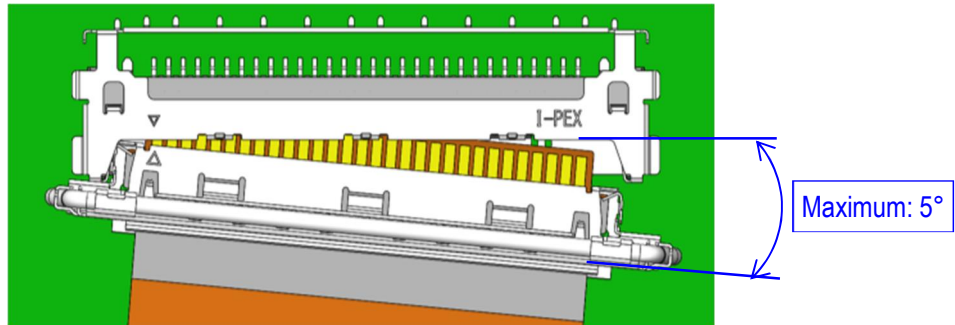
Fig. 22 Maximum Horizontal Removal Angle
