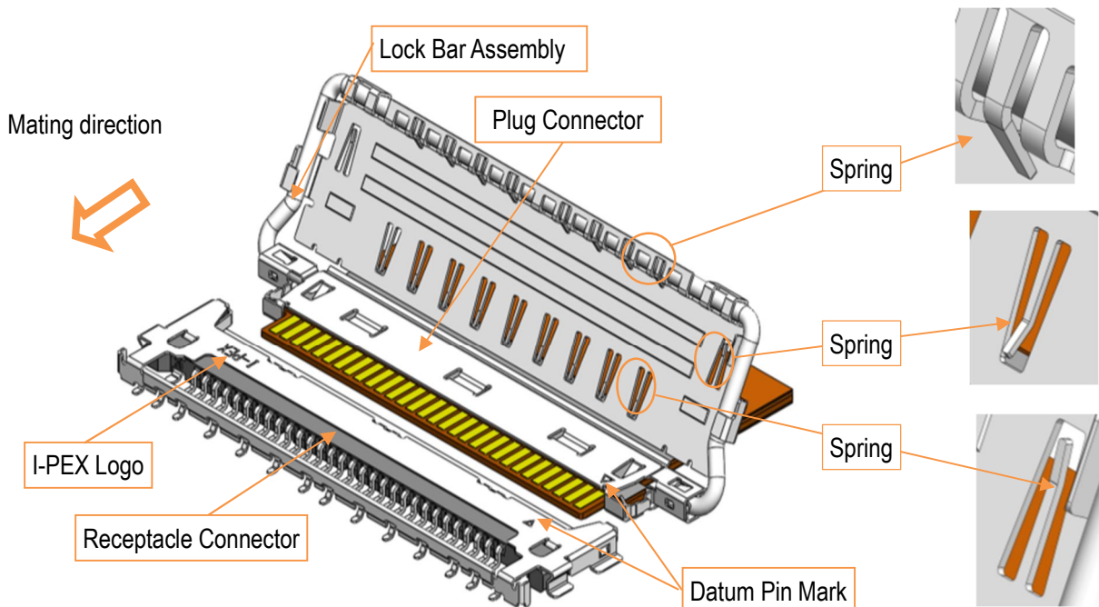
Fig. 3 Names of the Connector Parts
