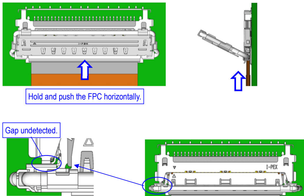
Fig. 7 Correct Insertion Method
