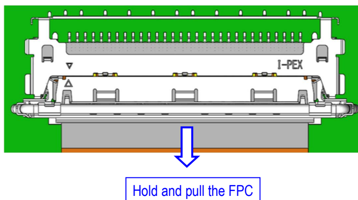
Fig. 21 Correct Removal Method
