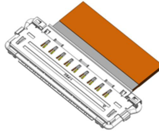
Fig. 1 Closed Shell Assembly with FPC
