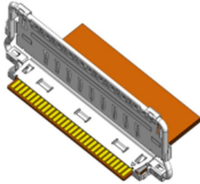
Fig. 2 Opened Shell Assembly with FPC
