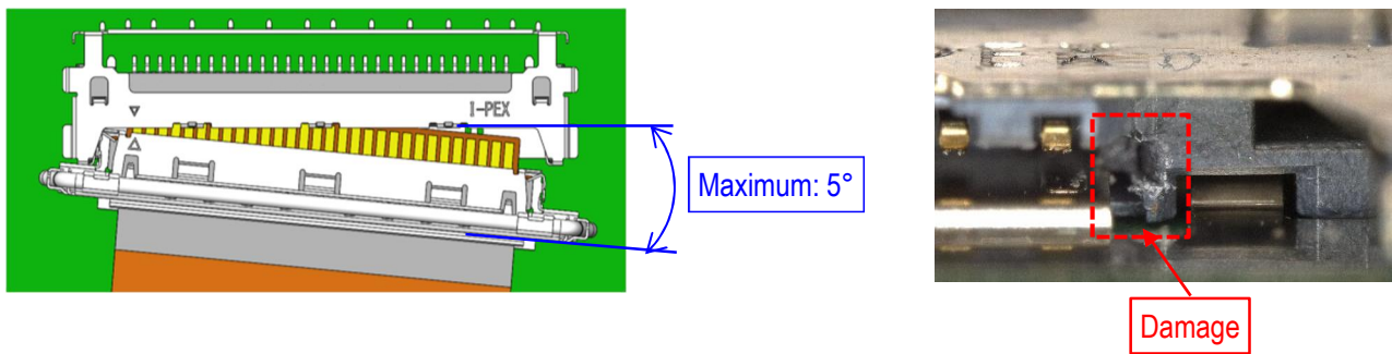
Fig. 11 Maximum Horizontal Insertion Angle
