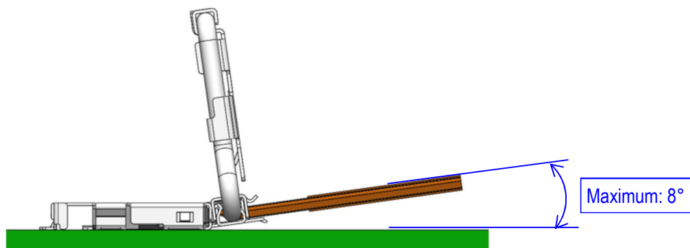
Fig. 6 Maximum Vertical Insertion Angle
