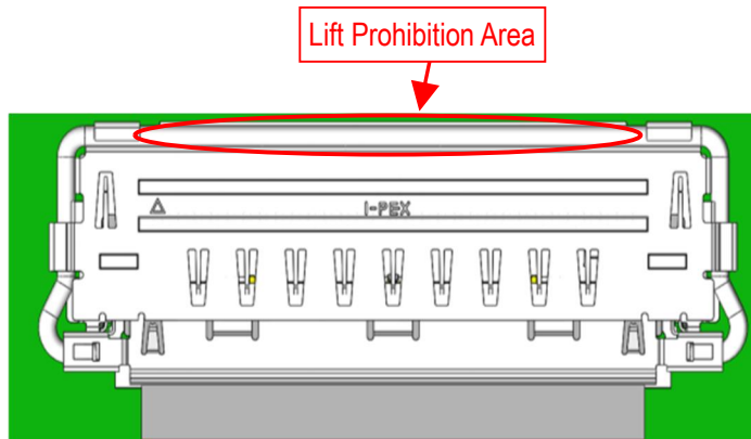
Fig. 20 Lift Prohibition Area
