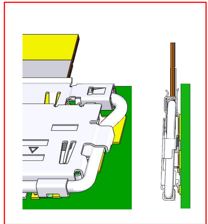
Fig. 18 Incorrectly Locked
