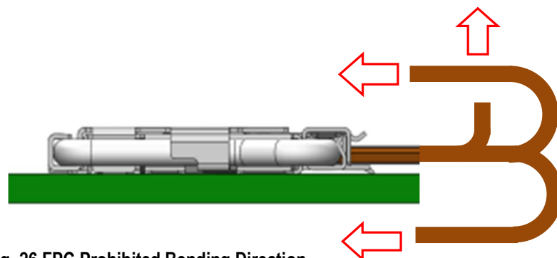
Fig. 26 FPC Prohibited Bending Direction
