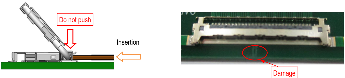
Fig. 15 Force Applying Prohibition
