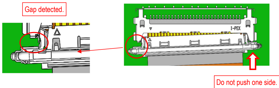
Fig. 8 Incorrect Insertion Check
