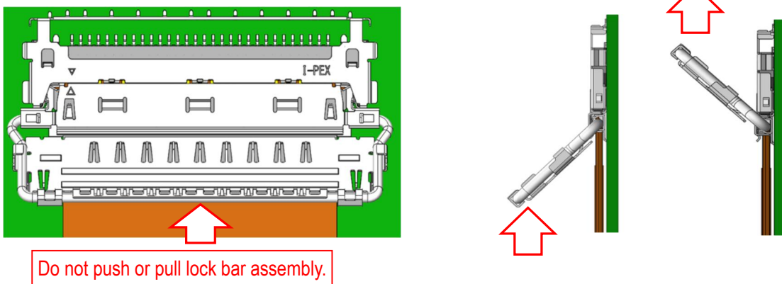
Fig. 14 Incorrect Insertion Method
