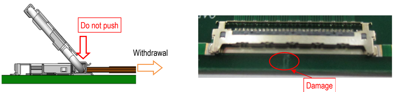
Fig. 24 Force Applying Prohibition
