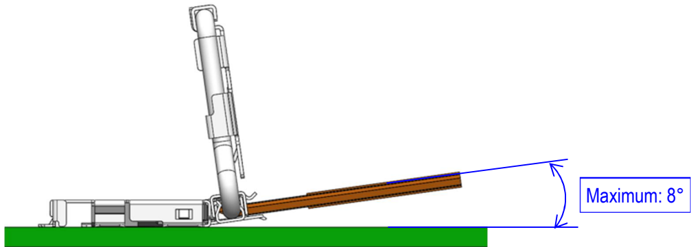
Fig. 13 Maximum Vertical Insertion Angle at Pre-insertion
