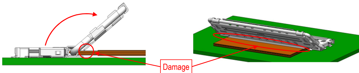
Fig. 12 The Lock Bar Opening Limitation
