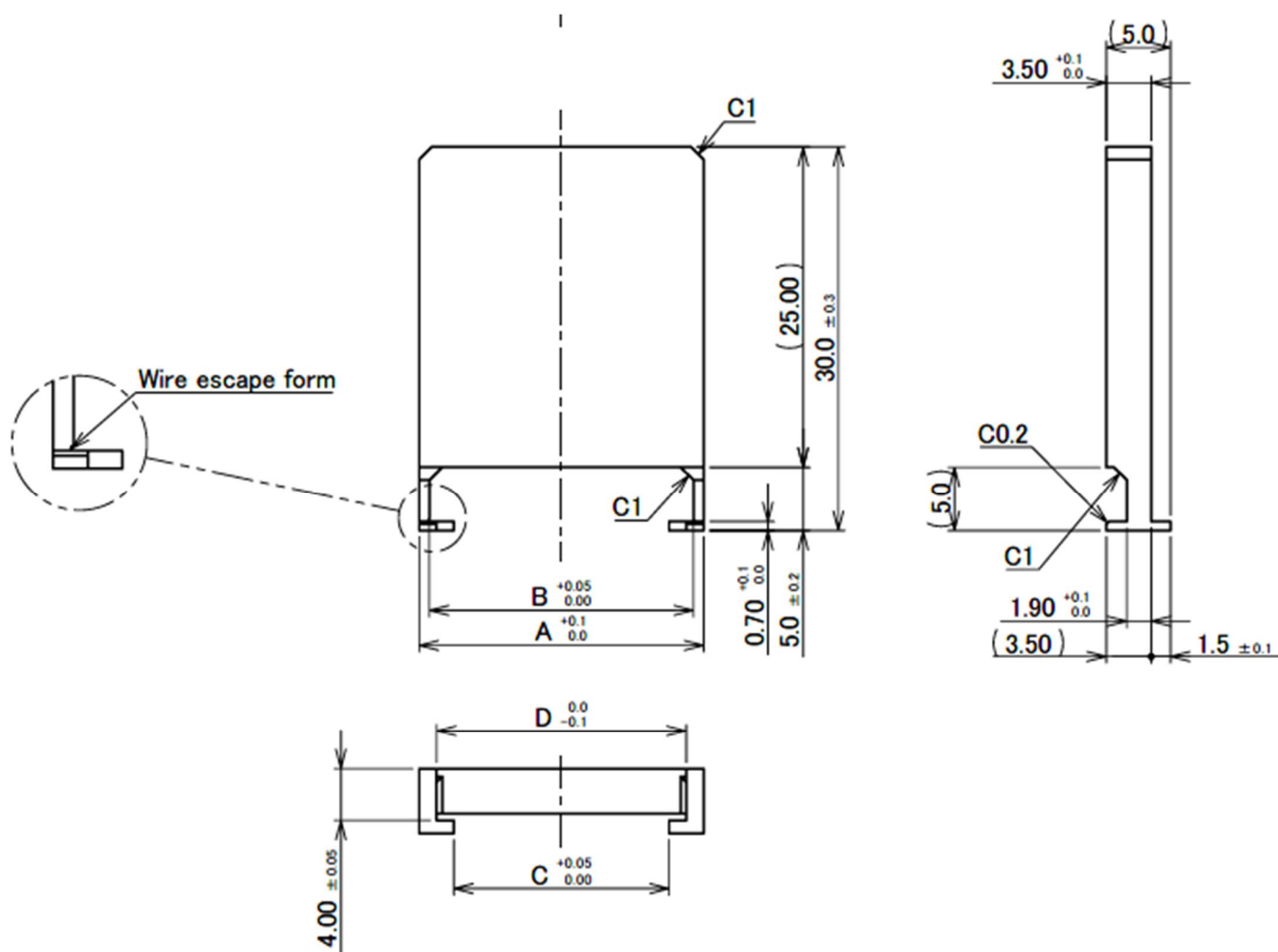
Fig.20 Reference: Plug Pull Jig
