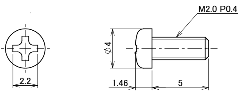
SCREW 90042-001 (S = 5/1)
