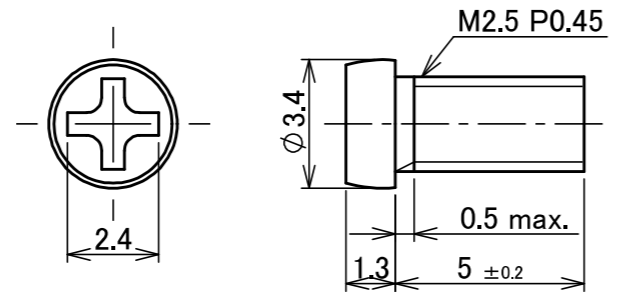
SCREW 90023-001 (S= 5:1)
