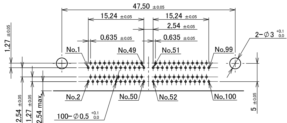
RECOMMENDED FOOTPRINT PATTERN t=1.6 \pm 0.1 (100P ONLY)
