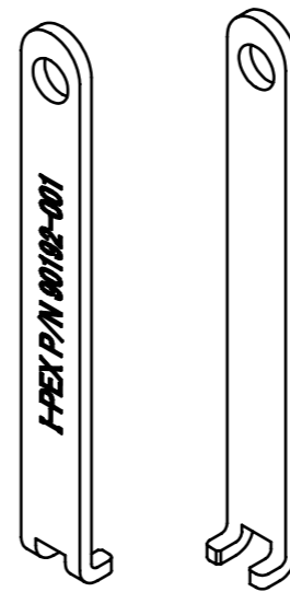
FRONT SIDE BACK SIDE MHF I UNMATING TOOL PART NO. 90192-001
