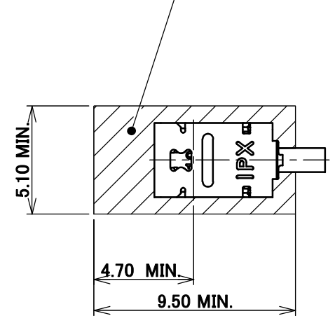
MATING AND LOCK CONDITION WITH MHF I LK HARNESS NARROW PITCH
