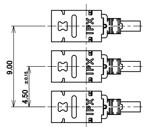
MHF I LK HARNESS UNLOCK CONDITION NARROW PITCH DIMENSIONS
