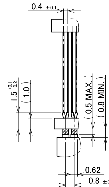
RECOMMENDED TWINAX CABLE DIM. (AWG#40)
