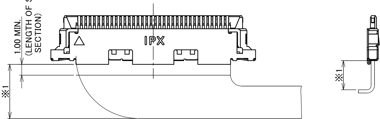
REFERENCE CABLE BENDING DIMENSIONS
