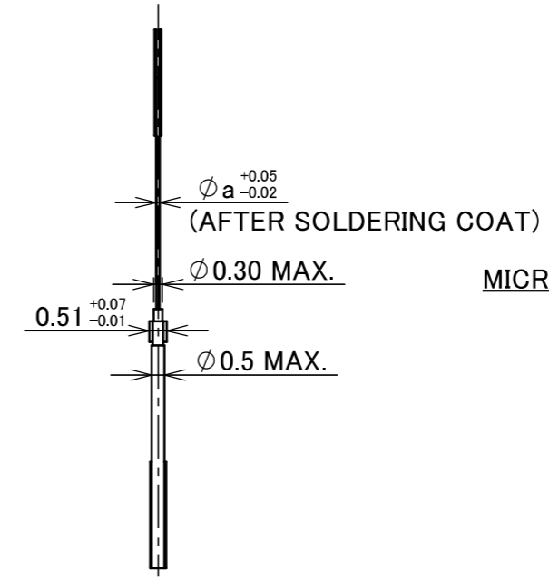
MICRO-COAXIAL CABLE AWG#**
