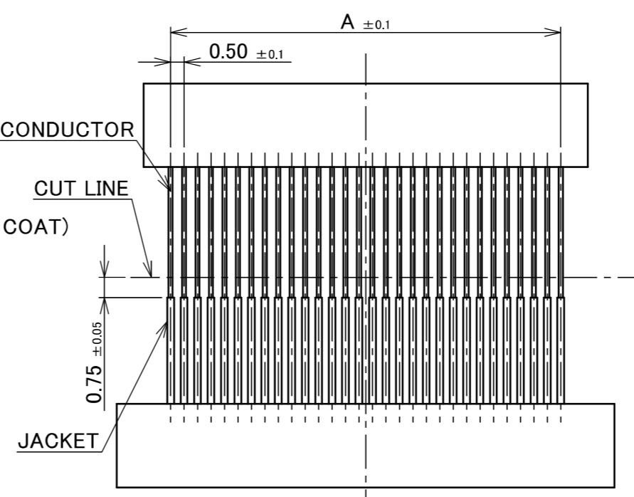
RECOMMENDED DISCRETE WIRE DIMENSION
