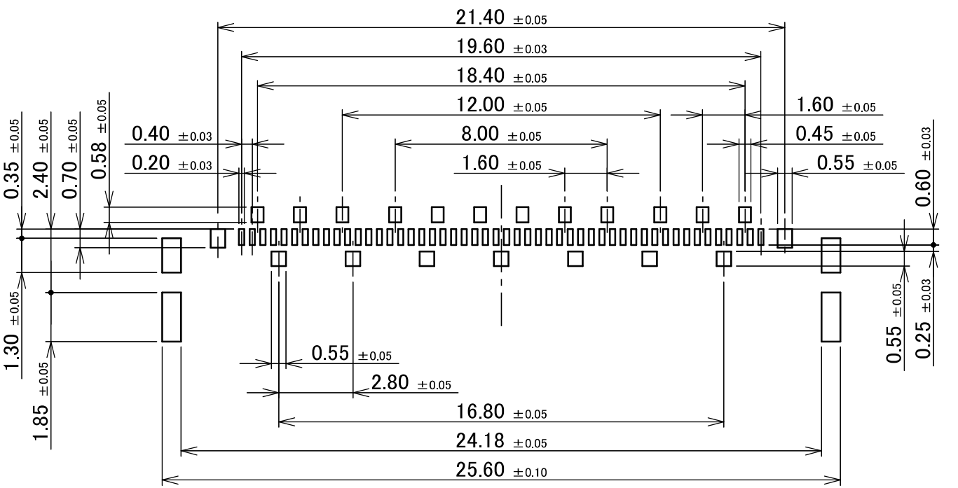
50P RECOMMENDED METAL MASK LAYOUT METAL MASK THICKNESS : t=0.12mm
