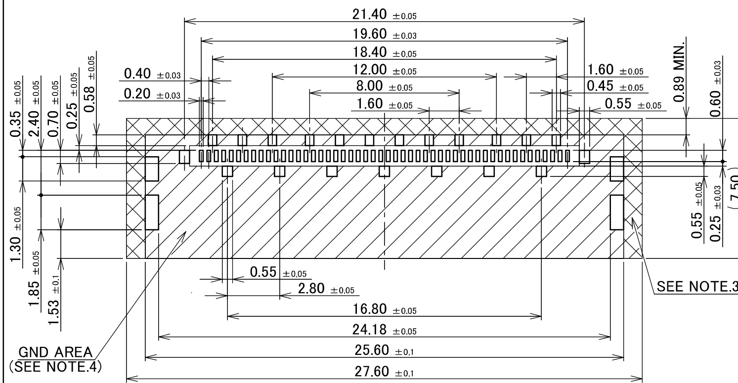
50P RECOMMENDED FOOTPRINT PATTERN LAYOUT
