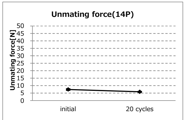
Graph-6. A change of unmating force (14P)
