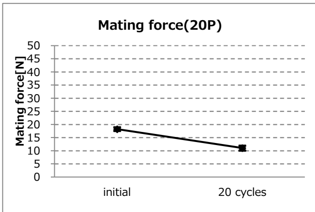
Graph-9. A change of mating force (20P)
