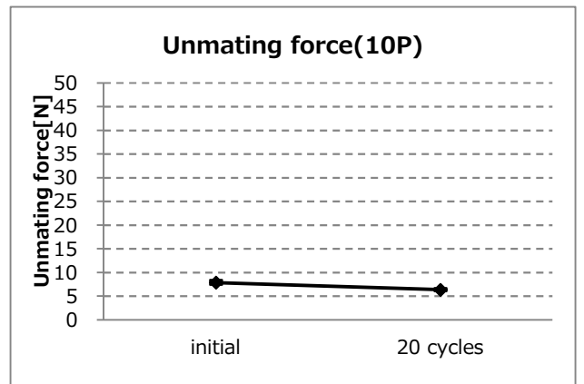
Graph-4. A change of unmating force (10P)
