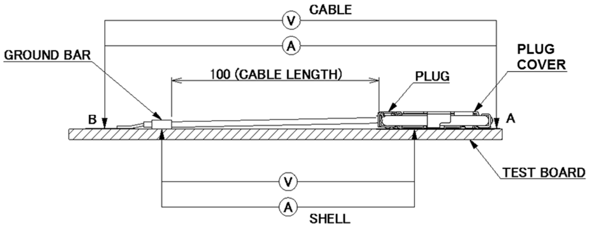
図1 接触抵抗 (Fig.1 Contact Resistance)
